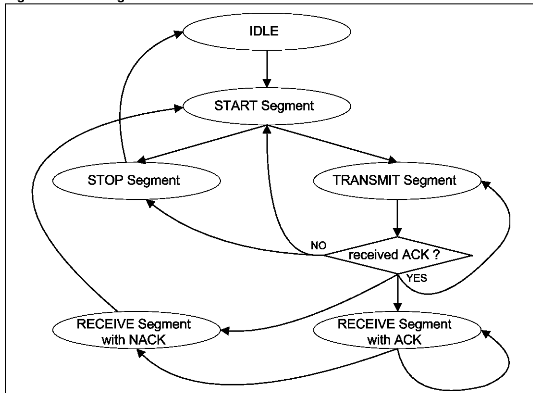
Figure 7. I 2 C segment transitions
